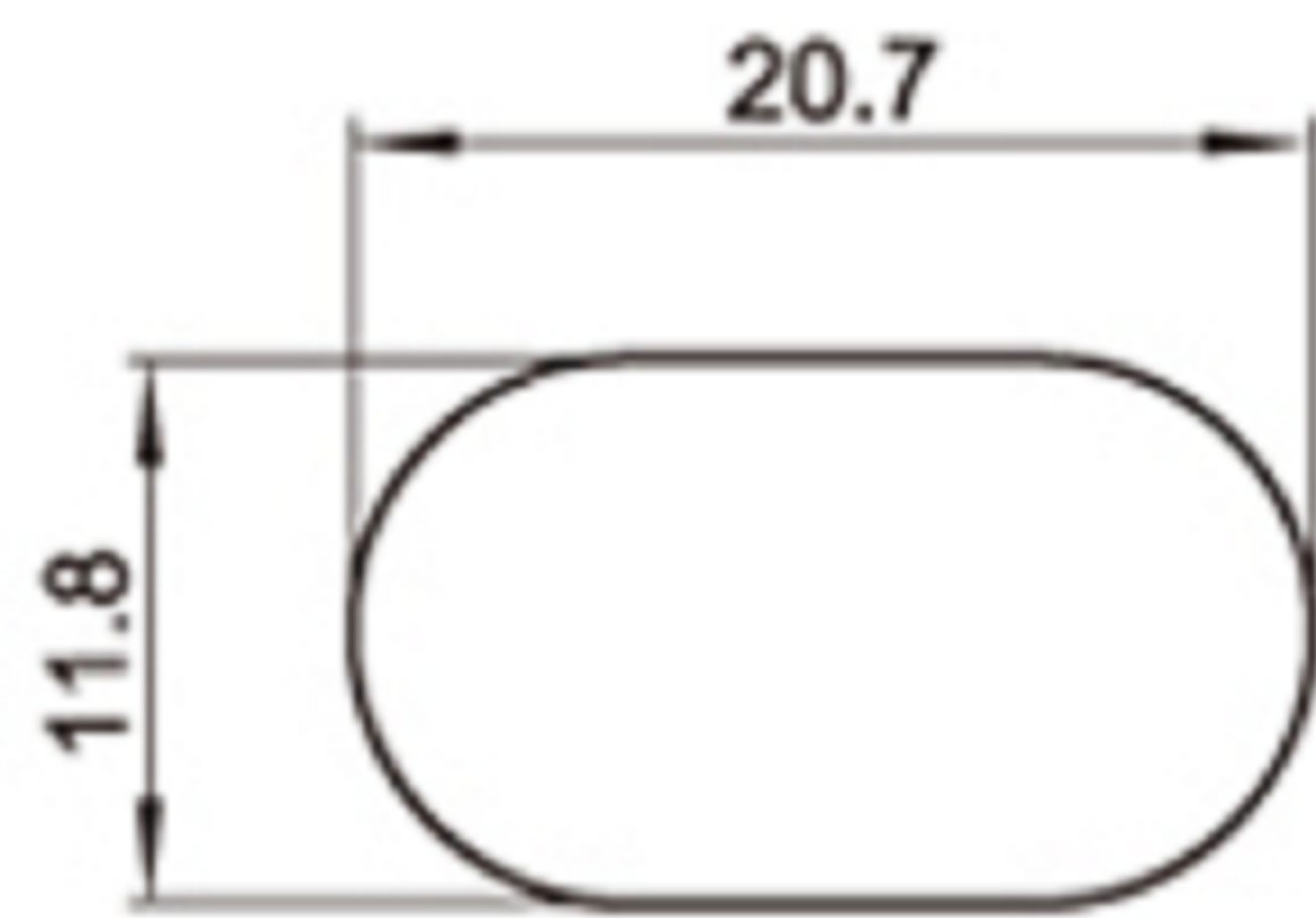
PANEL CUT-OUT
